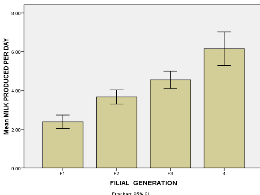
Figure 2: Mean daily milk yield (kg) among filial generations
